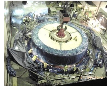
San Esteban II Hydroelectric Power Plant, Spain
