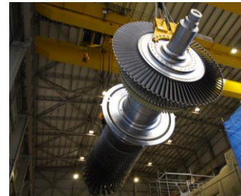
Triple C Inspection on the Turbines and Alternator of the Soto V CCPP, Spain
